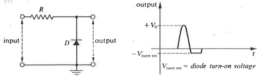
(b) clipping circuit
