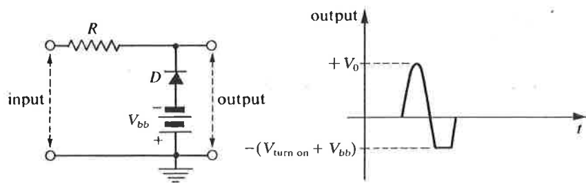
(c) clipping circuit with battery
